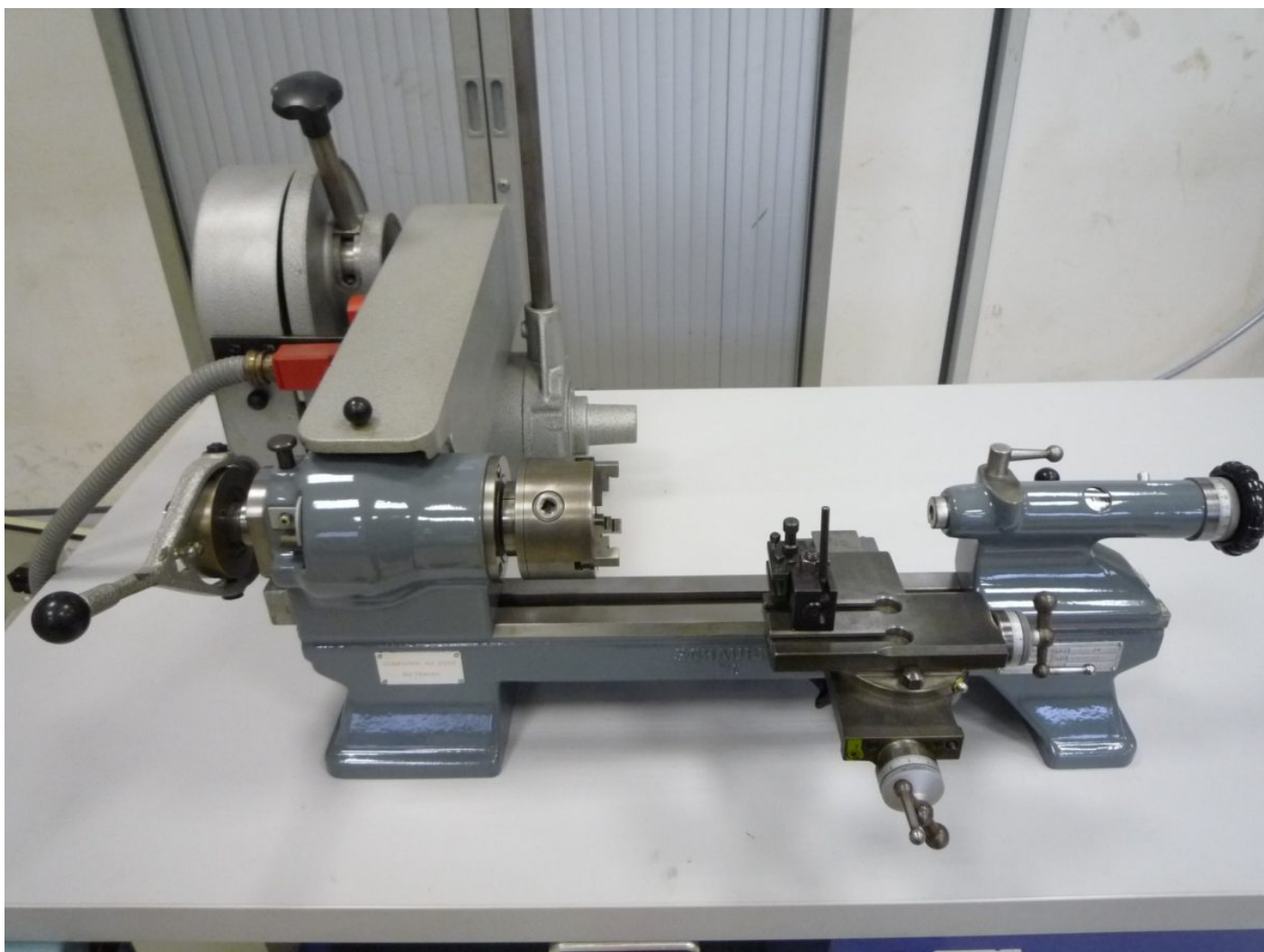
Lathe SCHAUBLIN 70
